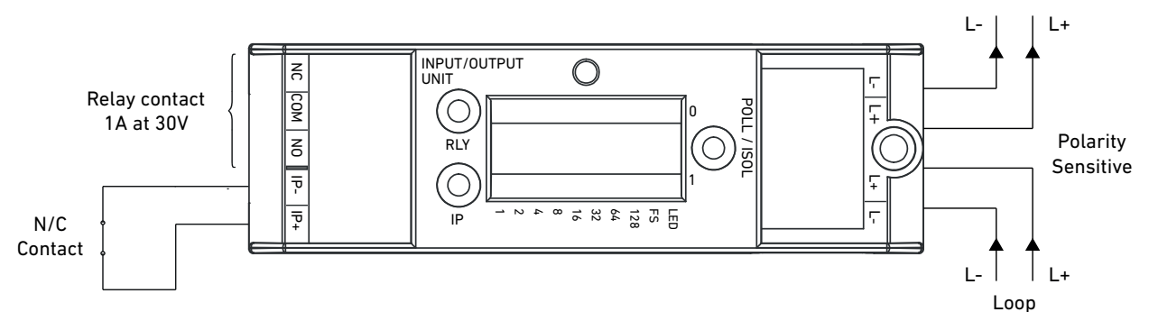
Figure 4: Intelligent Twin Input/Output Unit normally closed monitoring mode connectivity diagram (compatible with CoreProtocol only)
