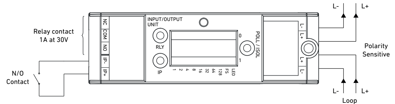
Figure 3: Intelligent Twin Input/Output Unit normally open monitoring mode connectivity diagram (compatible with CoreProtocol only)
