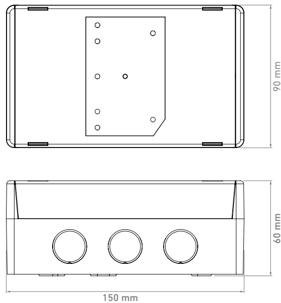
Figure 1: Intelligent Twin Switch Monitor dimensional drawing
