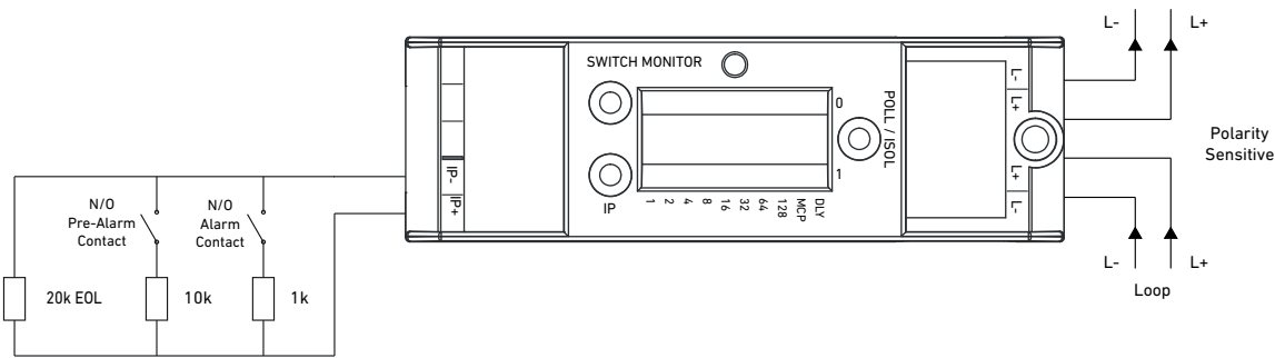
Figure 2: Intelligent Twin Switch Monitor standard resistive monitoring mode connectivity diagram
